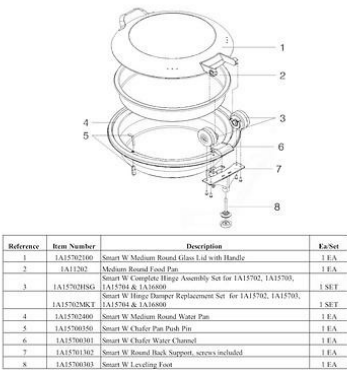
SMART BUFFET WARE Item No: 1A15702 Description: SMART W ROUND MEDIUM CHAFING DISH WITH GLASS LID
